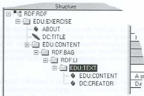
Figure 33: This the DOM of our RDF document. The example document was read by Microsoft's XML notepad. The XML notepad doesn't know about RDF and doesn't treat the RDF document any differently from any other XML document.
