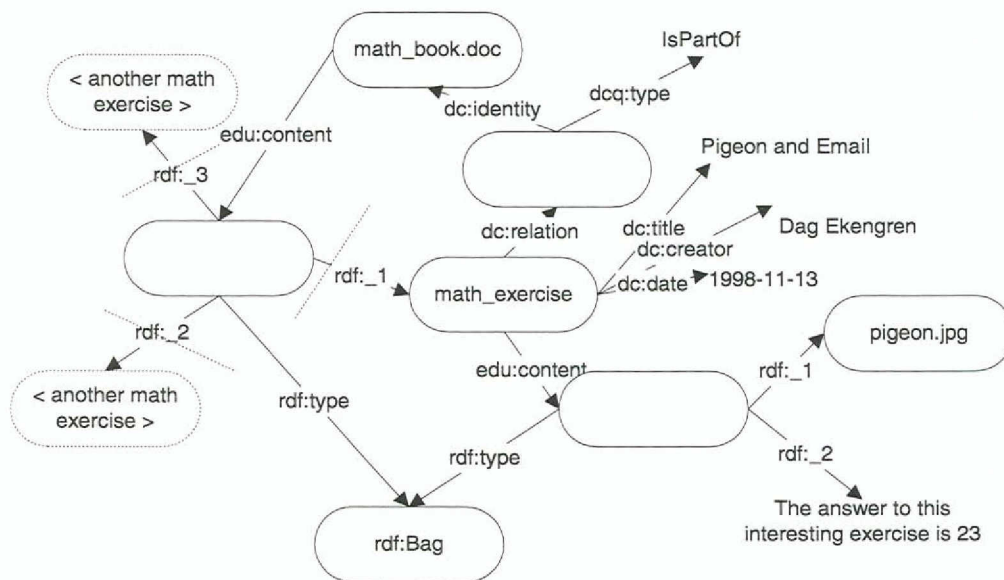
Figure 11: The Description construct. The collection of statements called a description does not need a special construct in the data model. A bag container is used to indicate that a set of statements belongs to the same description.
