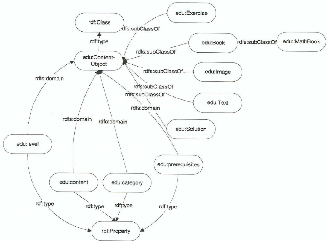
Figure 22: RDF schema for the edu namespace
