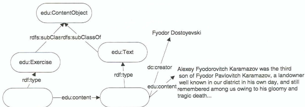
Figure 18 Invalid if the edu:content property's range is ContentObject .
