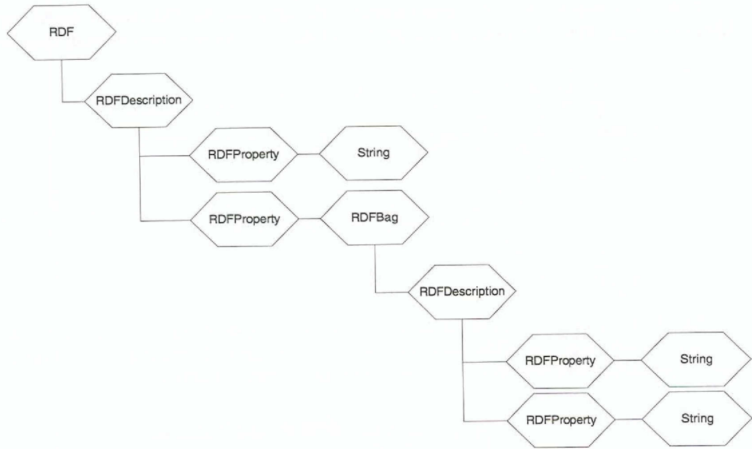
Figure 34: The RDF data model built from our sample RDF document. The boxes are Java object instances of the named classes. The RDF document's root node is of class RDF . It contains one RDFDescription instance (describing math_exercise ). The RDFDescription instance is parent for two RDFProperty instances. The first instance (corresponding to dc:title ) has a string value. The other property instance ( edu:content ) has an RDF bag as value.
