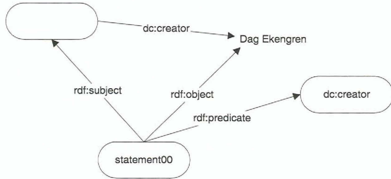
Figure 9: The statement has been reified
