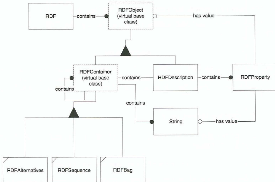
Figure 39: The RDF parser's class hierarchy
