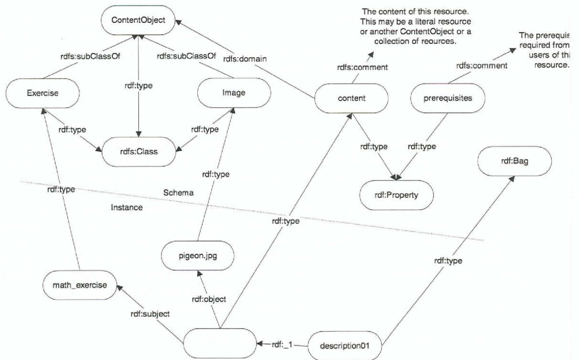
Figure 17: This is part of the schema definition for eduschema . Note that the schema is part of the RDF data model for the math exercise. We have defined Exercise and Image as subclasses of a ContentObject class and we have constrained the content property so that it can only be used on instances of ContentObject (or subclasses thereof). The dotted line is the division between schema and instance.
