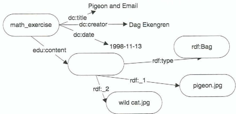
Figure 7: We have used a Bag to collect wild cat.jpg and pigeon.jpg.
